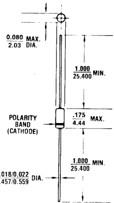
FIGURE 1 All dimensions in INCH m.m.
